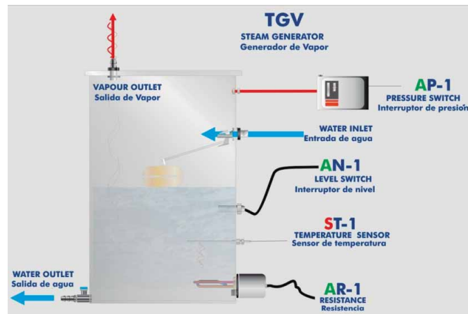
Process diagram and unit elements allocation
