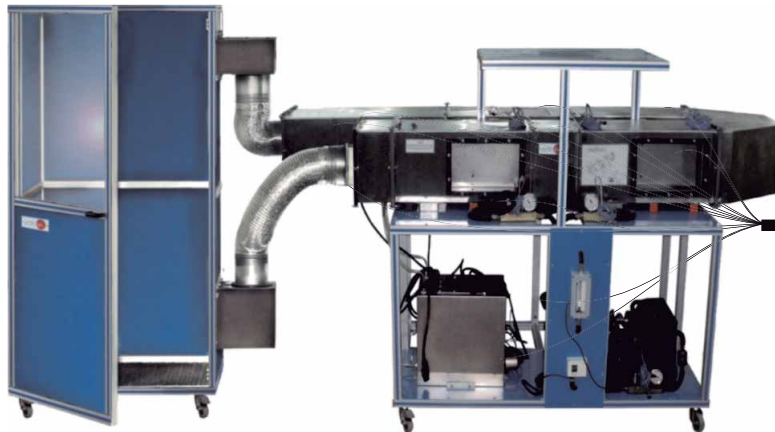
① Unit: TACC. Air Conditioning Unit with Climatic Chamber and Water Chiller
