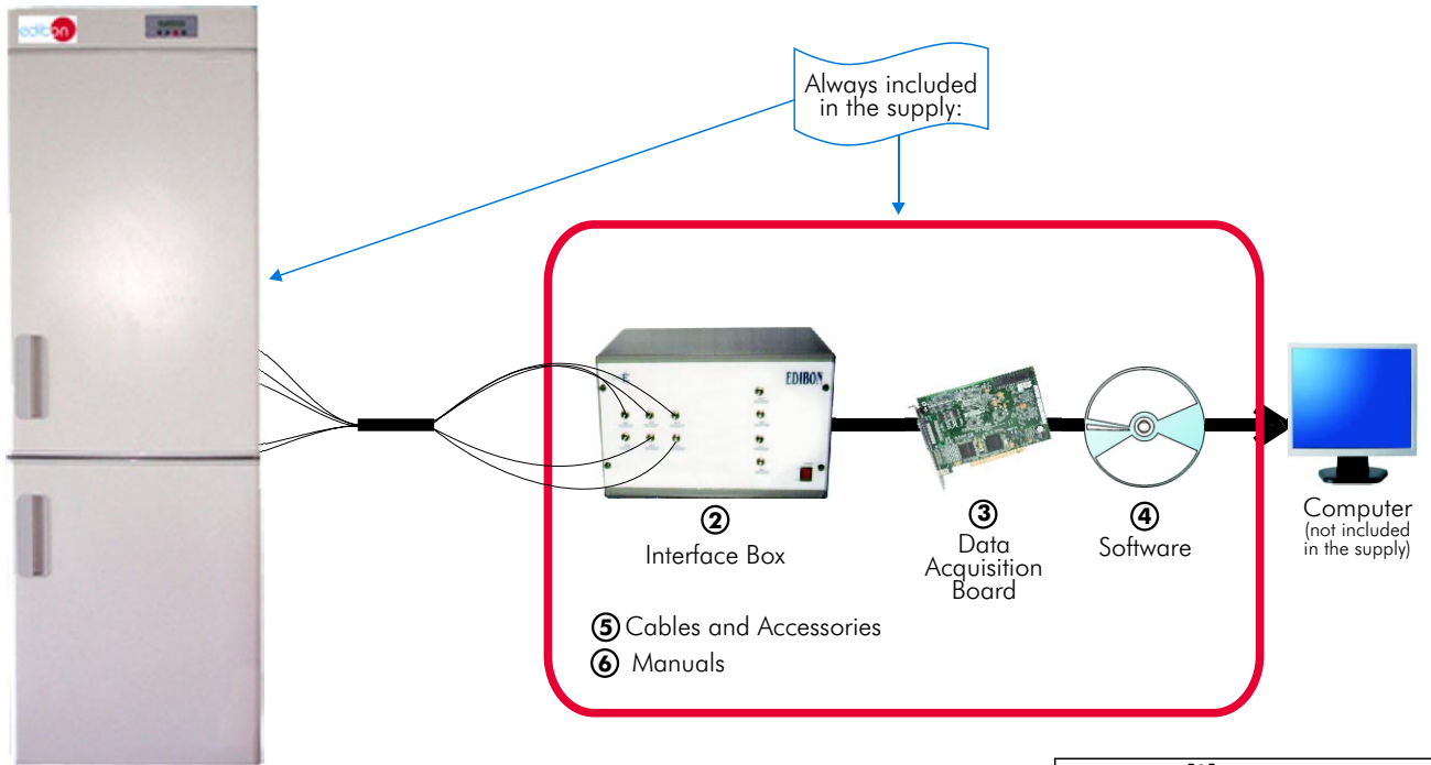
① Unit: TRD2PC. Two Doors Domestic Refrigeration System Trainer
